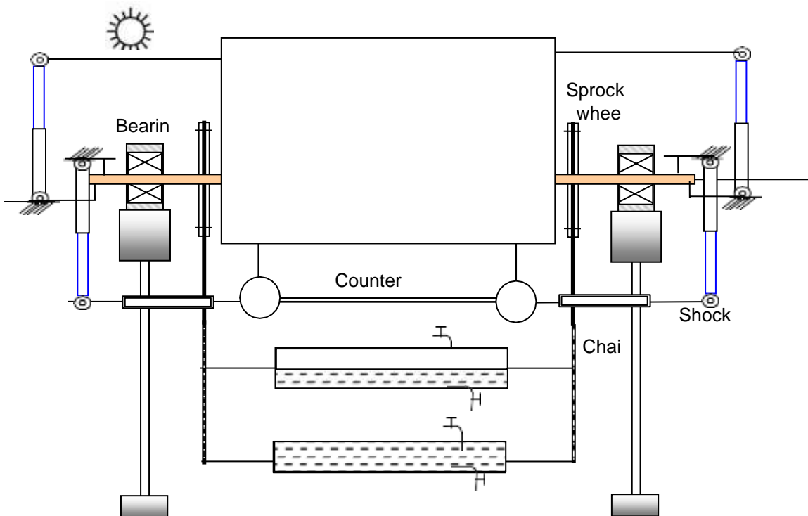
Fig. 3 Eccentric suspension (a) for collector and (b) for counter weight
