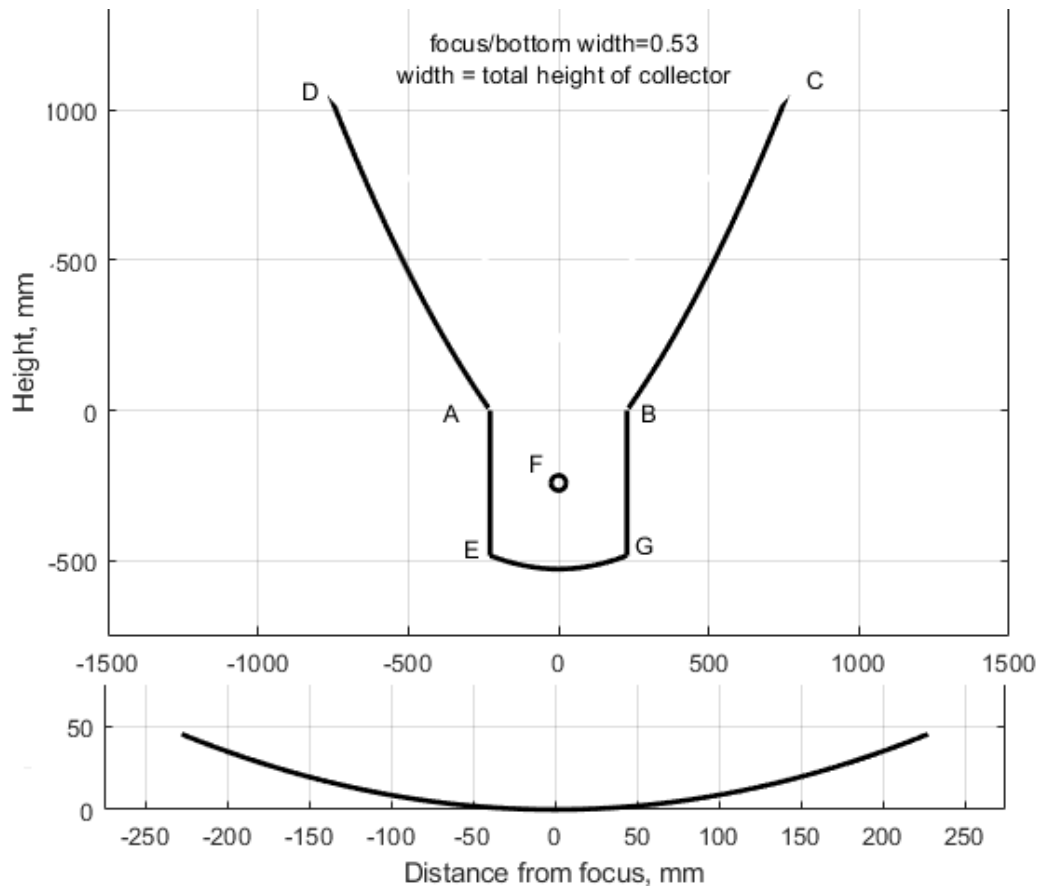
Fig. 1 Multi reflector compound parabolic collector
